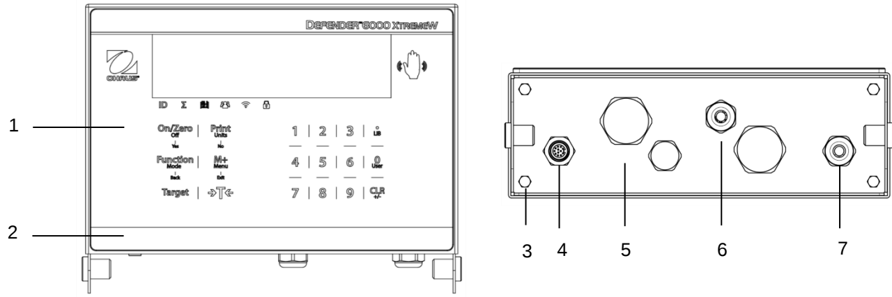
Figure 1-2 i-DT61XWE Indicator
