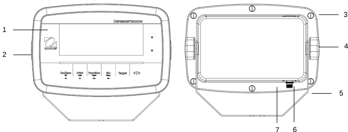
Figur 1-1 i-DT61PW-indikator
